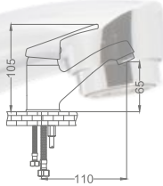
Line Mix Aplike Eviye Bataryası Line Mix Ornamented Kitchen Faucet
