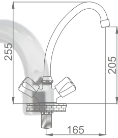
Nida Klasik Köprülü Lavabo Bataryası Nida Classic Bridge Basin Faucet
