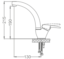
Line Mix Eviye Bataryası Line Mix Kitchen Faucet
