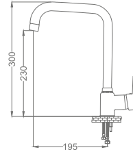
Didim Mix Kugulavabo Bataryası Didim Mix Swan Neck Kitchen Faucet
