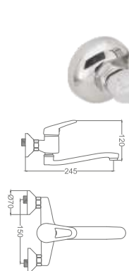
Line Mix Aplike Eviye Bataryası Line Mix Ornamented Kitchen Faucet
