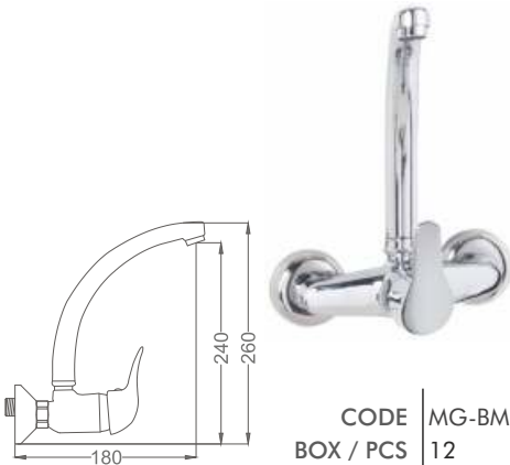
Mega Mix Ters Aplike Eviye Bataryası Mega Mix Omamented Kitchen Faucet
