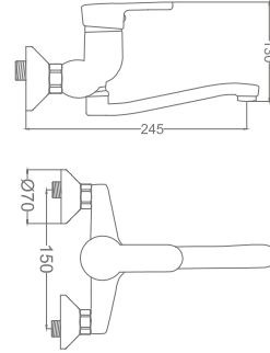
City Mix Aplik Eviye Bataryası City Mix Ornament Kitchen Faucet
