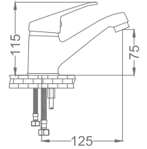
Mega mix Aplike Eviye Bataryası Mega Mix Ornamented Kitchen Faucet
