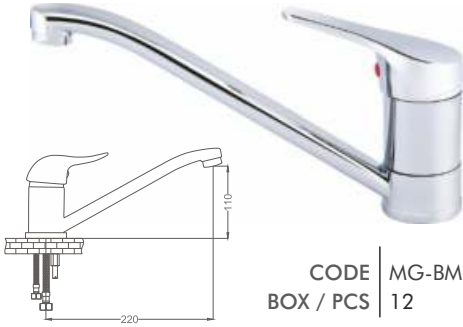
Mega Mix Ters Aplike Eviye Bataryası Mega Mix Omamented Kitchen Faucet
