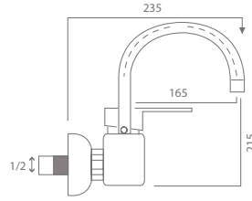
Snow Mix Kuyruklu Lavabo Bataryası Snow Mix With Tail Basin Mixer
