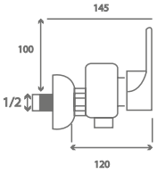
Truva Mix Kuyruklu Lavabo Bataryası Truva Mix With Tail Basin Mixer
