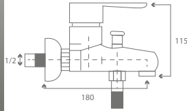
Truva Mix Aplike Eviye Bataryası Truva Mix Ornamented Kitchen Faucet
